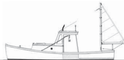
N° 77A—1:20 Lobster boat: Part 1 June 2006
