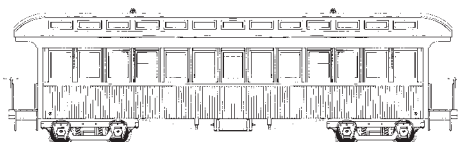
N° 55—1:20.3 narrow-gauge coach April 2002
