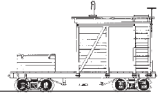
N° 62—Work caboose, 1:20 December 2003
