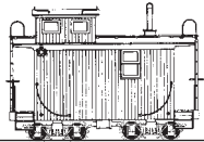
N° 63—Short caboose, 1:20 February 2004
