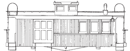
N° 71—1:20 Drivers' caboose June 2005
